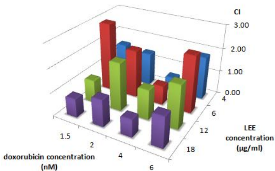
Figure 3. Diagram of combinational effect of LEE and doxorubicin against CI value. CI value below 0.9 shows synergicity.
